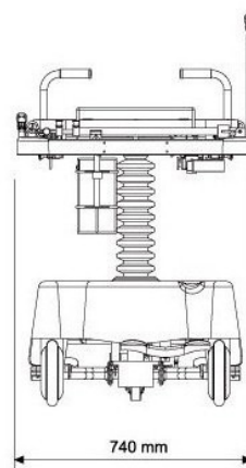
Right view
